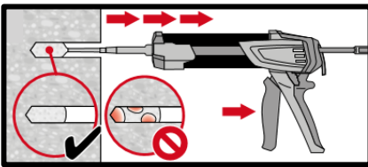
Injection method for drill hole
