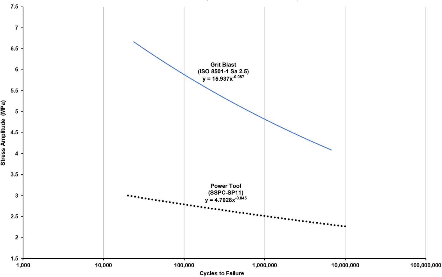
ISO 9664 – Belzona 7311 Cycles to Failure vs. Stress Amplitude
