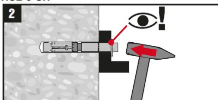
FIGURE 5—MANUFACTURER'S PRINTED INSTALLATION INSTRUCTIONS
