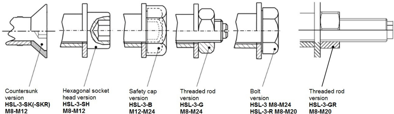
FIGURE 2—HEAD STYLES OF THE HSL-3 and HSL-3-R
