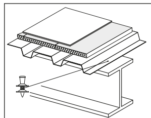
Roof decking
