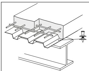
Floor decking
