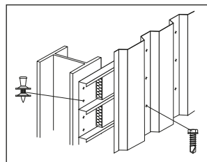
Wall liners
